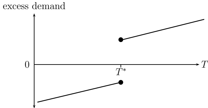
Figure 5: The symmetric excess demand correspondence jumps over the market-clearing level when u(x) = x^{0.3} , c(q) = 0.1 + q^{1.5} , \beta = 0.98 , and \pi = 0.01445 .
