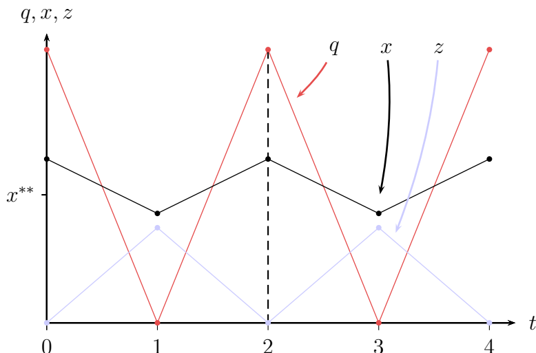
Figure 3: A money cycle with over-production and over-consumption, with u(x) = x^{0.3} , c(q) = 0.15 + q^{1.3} , \beta = 0.98 and \pi = 0.3 . Average consumption is above the efficient level, x^{**} .
