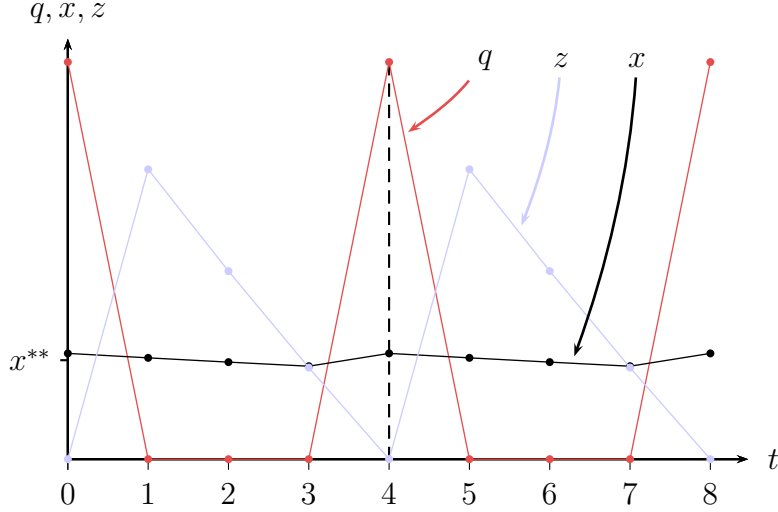
Figure 2: A simple money cycle. The symbols q , z and x denote production, real balances of money holdings, and consumption respectively. Consumption oscillates around the efficient level, x^{**} .
