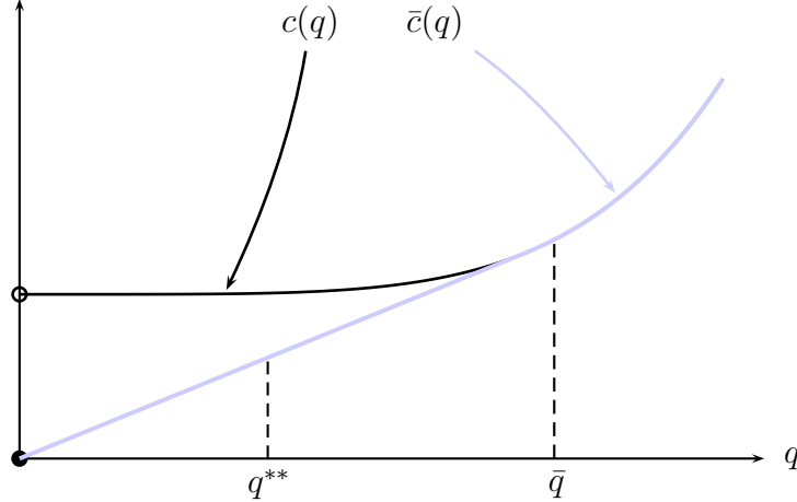
Figure 1: The convex hull of the cost function
